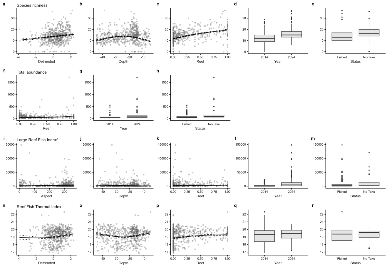
Figure C.5: Plots of the best model found to predict the probability of occurrence of key fish groups. Individual panes display the predicted relationships between model covariates and each demersal fish metric. Solid lines represent predicted Generalized Additive Model (GAM) fits with other variables held constant at their mean value, with year held at 2014 and zone status held at areas open to fishing. Dashed lines represent upper and lower standard error bounds around the prediction, and points represent the observed data from all survey years and zones. *Large Reef Fish Index representing the biomass of all fish greater than 20 cm (B20) has been adapted here for stereo-BRUV data by removing sharks and rays.
