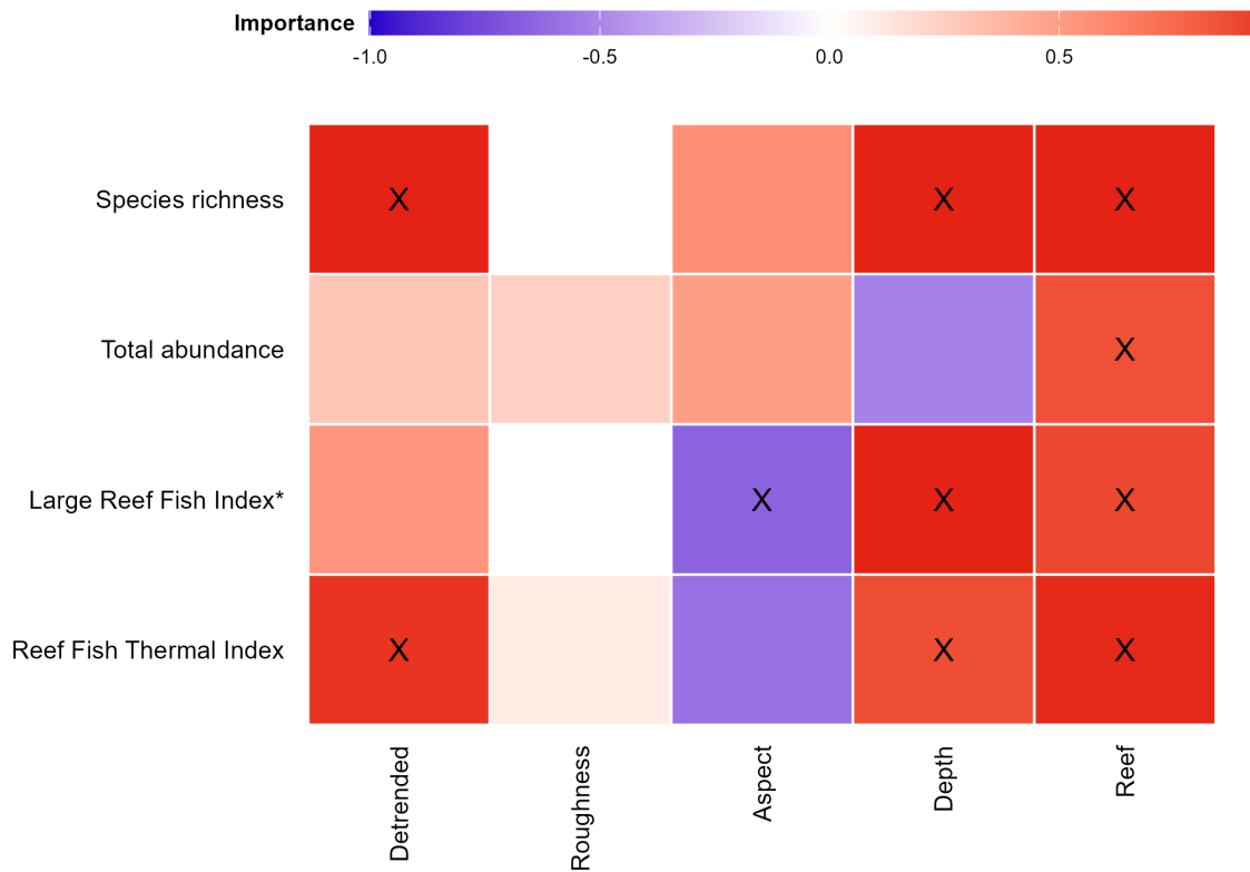
Figure C.4: Variable importance scores for predicting the probability of demersal fish metrics. Response variables included in the most parsimonious top model are indicated (X), with the colour gradient representing positive (red), zero (white) and negative (blue) relationships. Aspect is a circular variable, so the direction of its relationship should be read from the response curves rather than the colour gradient. *Large Reef Fish Index representing the biomass of all fish greater than 20 cm (B20) has been adapted here for stereo-BRUV data by removing sharks and rays.
