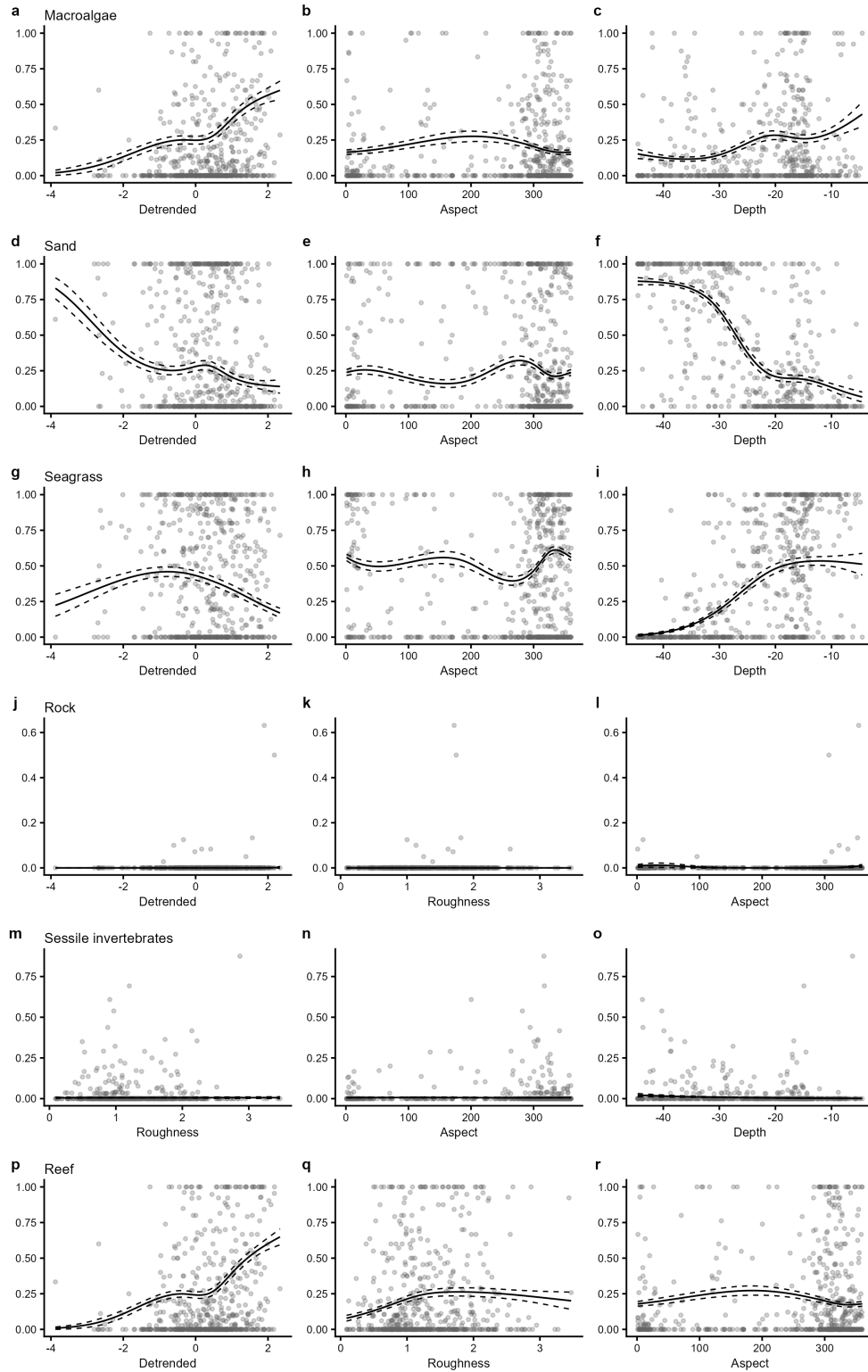
Figure C.3: Plots of the most parsimonious model found to predict the probability of occurrence of key habitat types. Individual panes display the predicted relationships between model covariates and the probability of occurrence of each habitat class. Solid lines represent predicted Generalized Additive Model (GAM) fits with other variables held constant at their mean value. Dashed lines represent upper and lower standard error bounds around the prediction, and points represent the observed data from all survey years.
